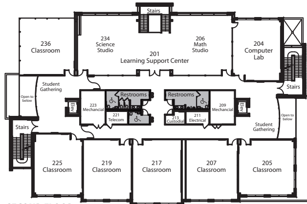
SECOND FLOOR
